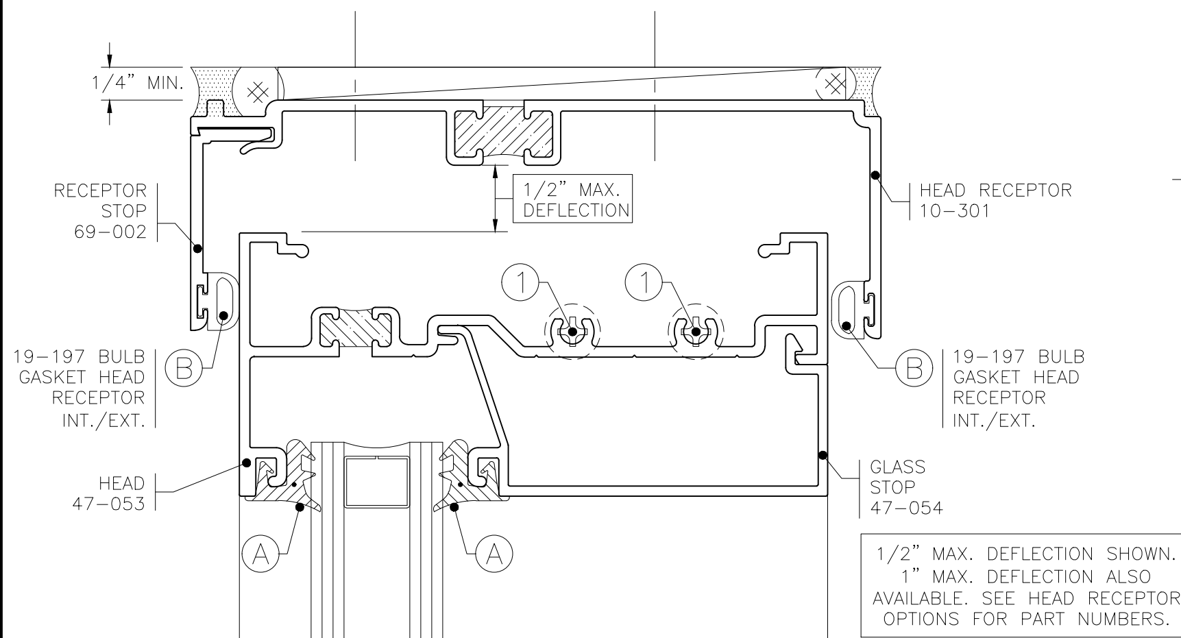
HEAD RECEPTOR
