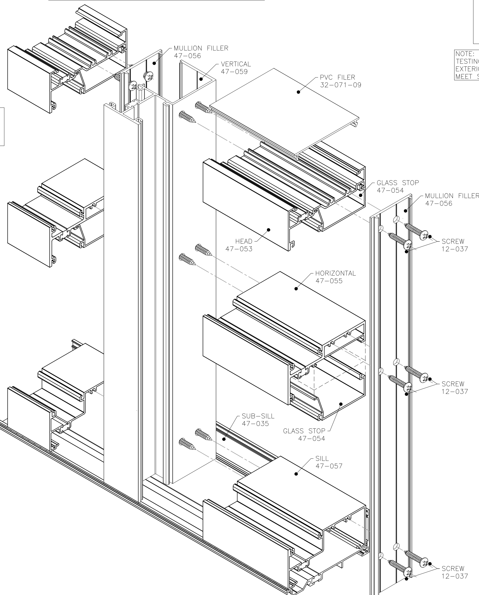
ASSEMBLY ISOMETRIC
