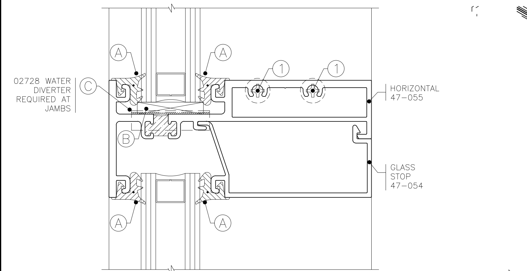
HORIZONTAL MULLION
