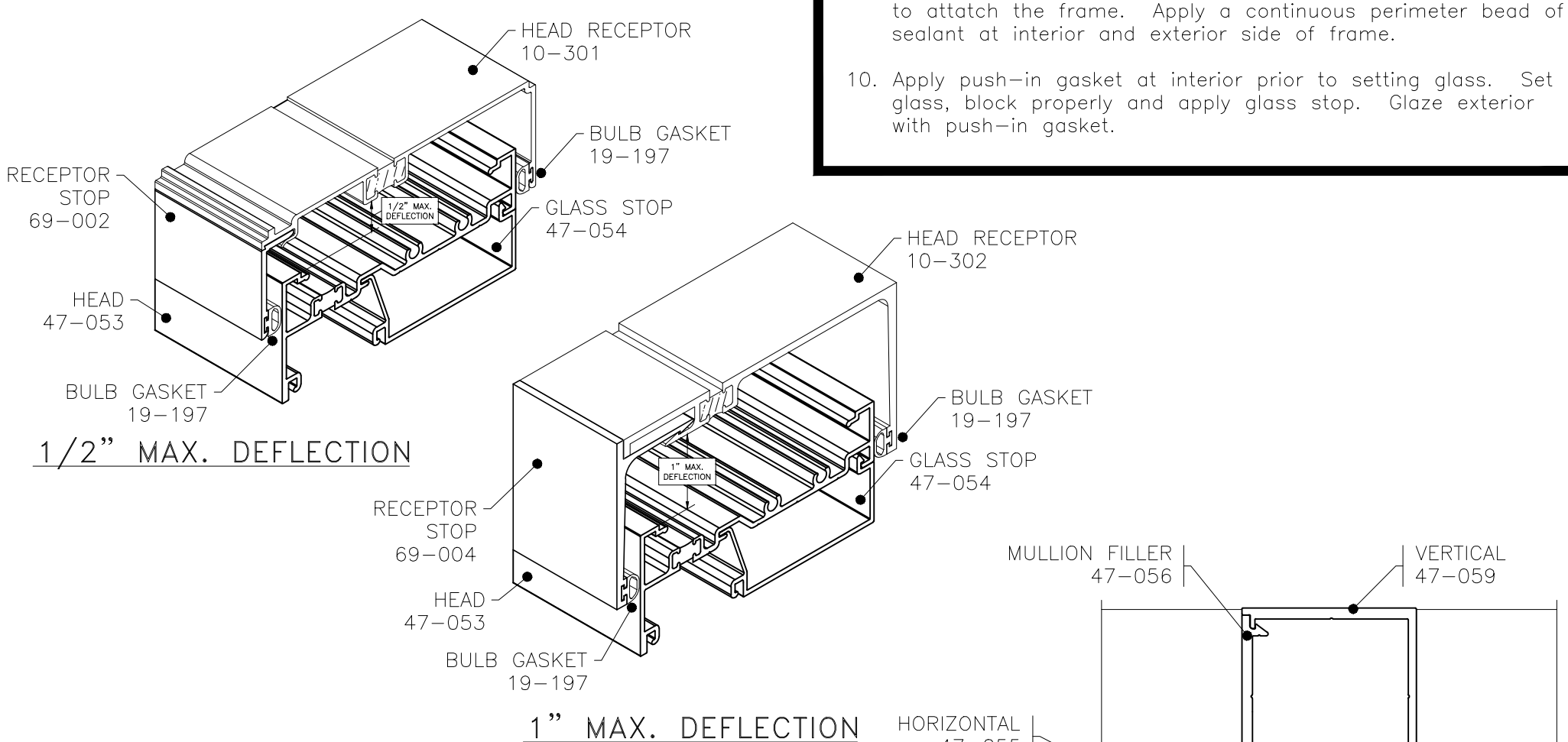
HEAD RECEPTOR OPTIONS
