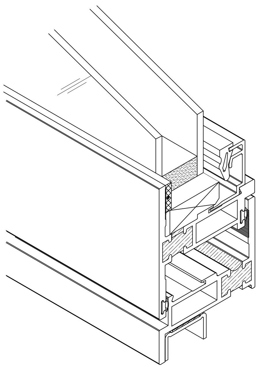
ISOMETRIC SILL SECTION
