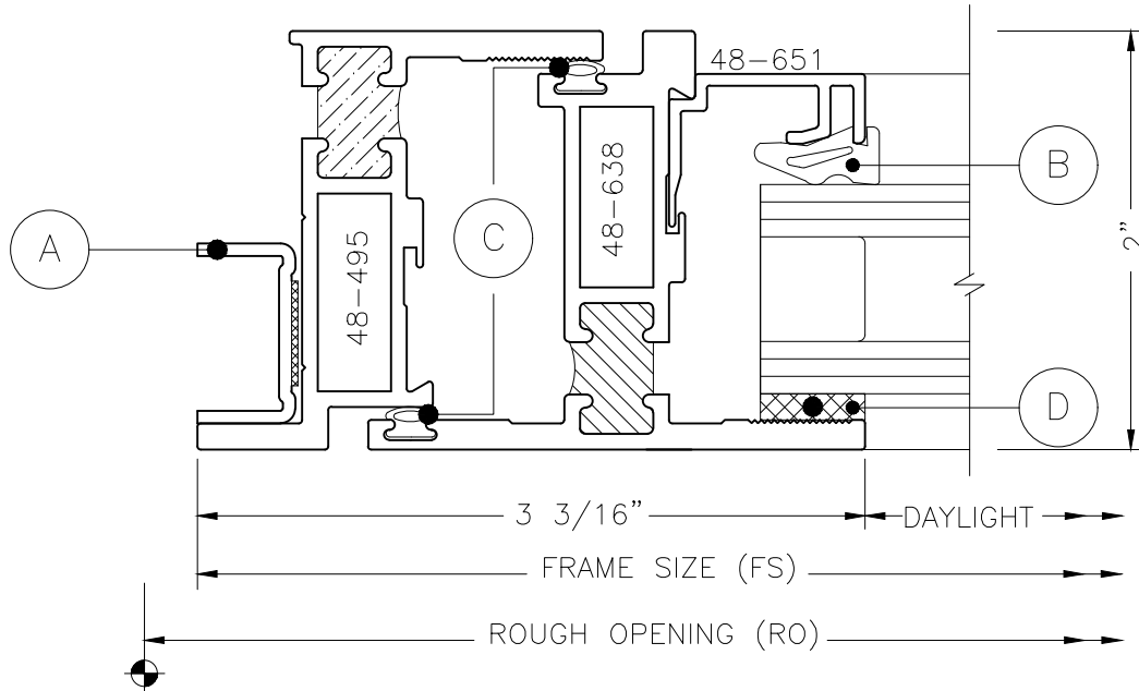
1/2" GLAZING LEG JAMB WITH GLAZING ADAPTOR
