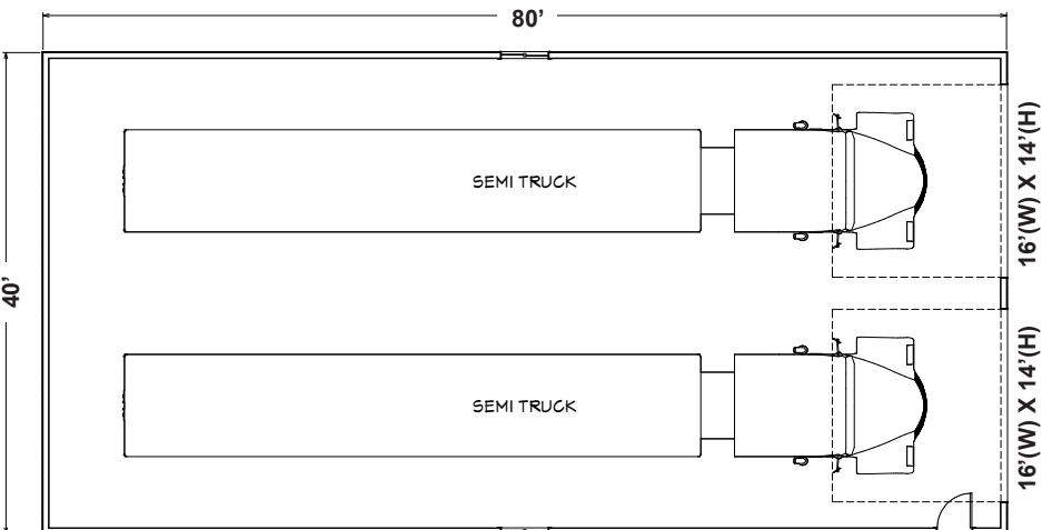
40'(W) x 80'(L) x 16' WALL
